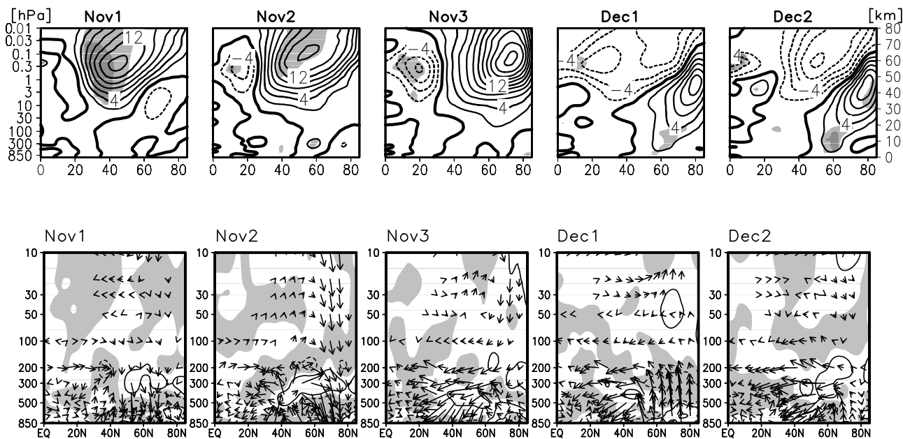
Figure 24. (top) Long-term 10 day mean differences of NH zonally averaged zonal wind between S_{max} and S_{min} from GCM experiments for 1–10 November (Nov1) and 11–20 November (Nov2) through to 11–20 December (Dec2). Contour interval is 2 \text{ m s}^{-1} . Light (heavy) shading indicates the 5% (1%) significance level calculated with a Student’s t test. (bottom) Corresponding plots for Eliassen-Palm flux vectors (arrows, scaled by the inverse of pressure) and its divergence. Only the 1 \text{ m}^{-1} \text{ s}^{-1} \text{ d}^{-1} contour is shown; negative values are shaded [from Matthes et al. , 2006].
